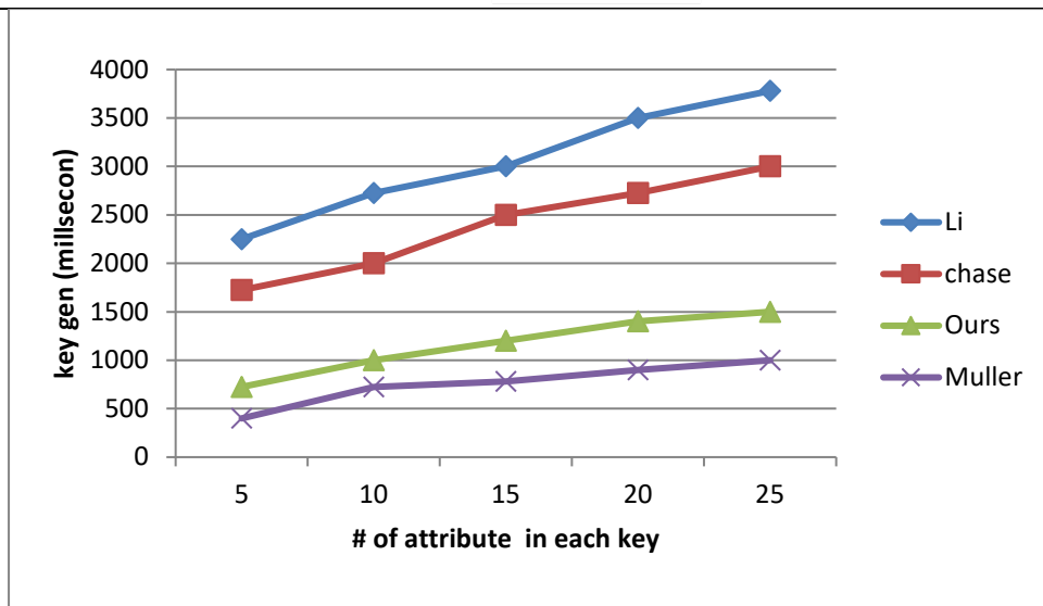
Figure 6 – # of attribute in each key and key gen time
