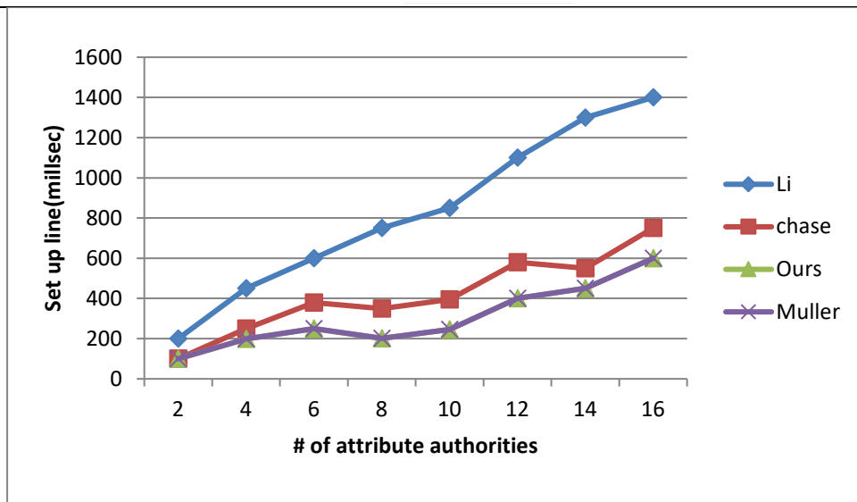
Figure 4 - # of attribute authorities and setup time
