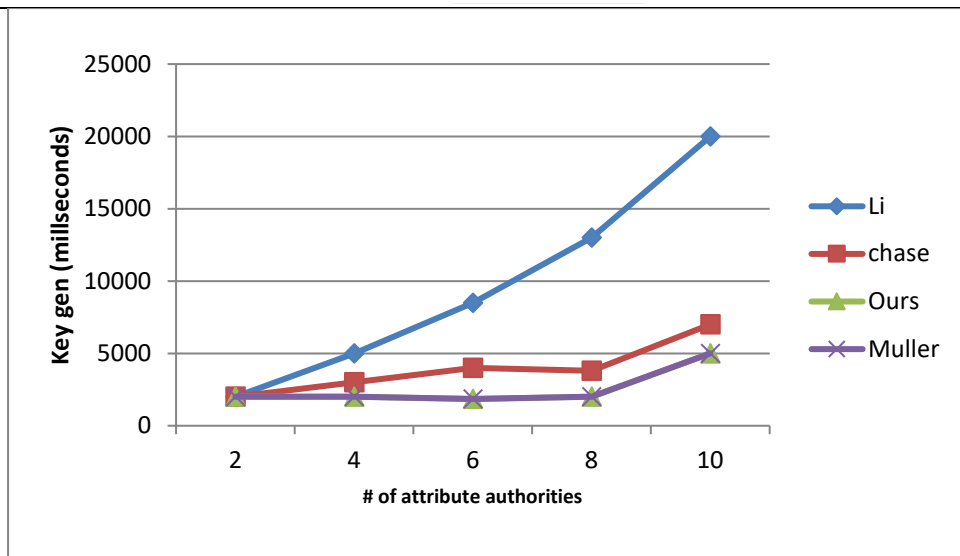
Figure 5 - # of attribute authorities vs. key gen time
